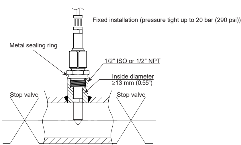
Fig. 31 Installation of the HTS801-T10 probe directly into the process
