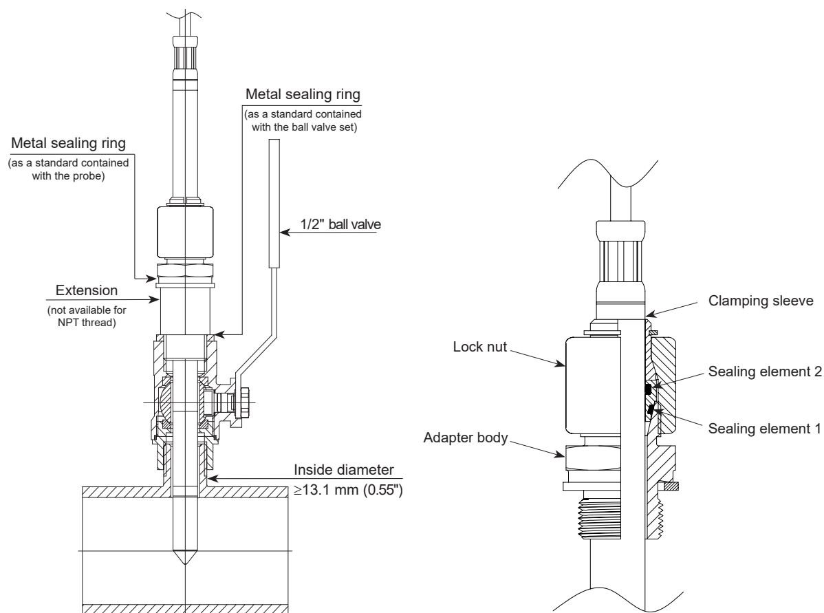
Fig. 32 Installation of the probe by utilizing the ball valve set
