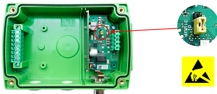
Fig. 24 Ethernet module - DHCP setting
