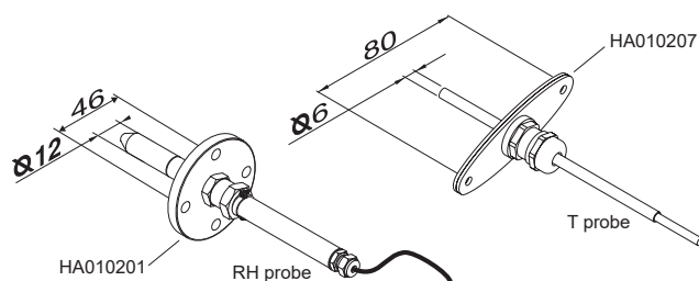
Fig. 34 Mounting of sensing probe with flange (accessory)
