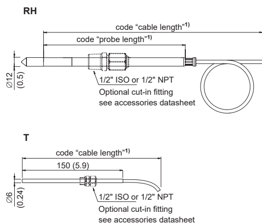
Fig. 33 Remote Sensing Probes Type T17
