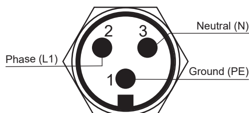
Fig. 40 Plug for power supply 100 - 240 V AC on stainless steel enclosure
