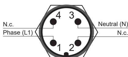
Fig. 39 Plug for power supply 100 - 240 V AC on polycarbonate enclosure
