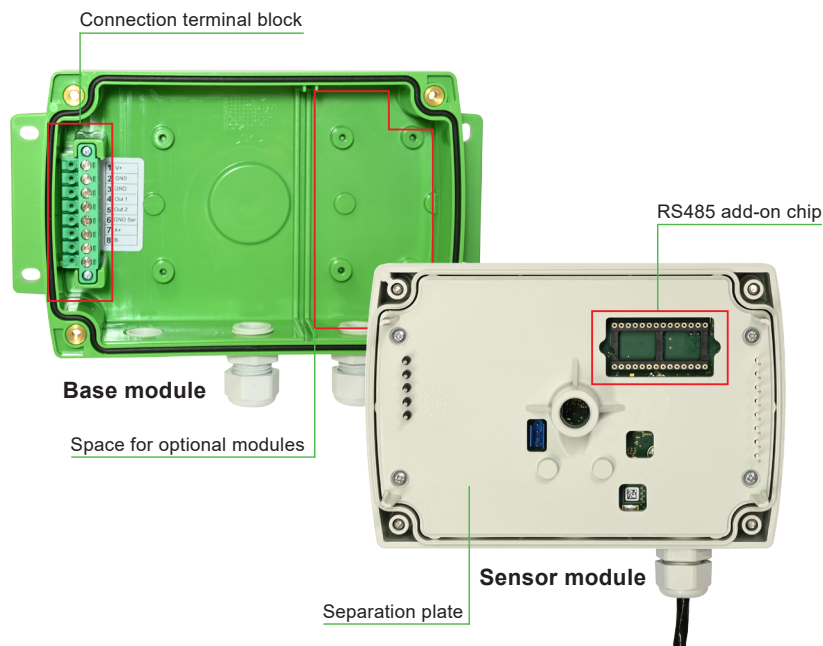
Fig. 3 HTS801 modular polycarbonate enclosure inside view
