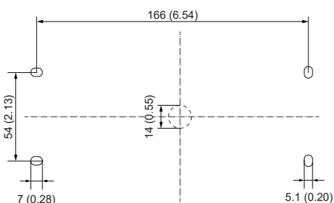
Fig. 25 Drilling pattern of polycarbonate enclosure
