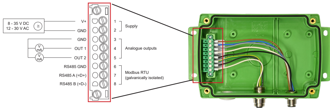
Fig. 36 Pin assignment on screw terminals for electrical connection via cable glands
