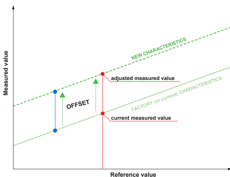
Fig. 45 1-point adjustment (offset)
