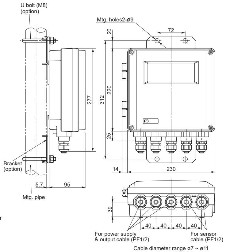
Flow transmitter : FSV...H (IP67)
