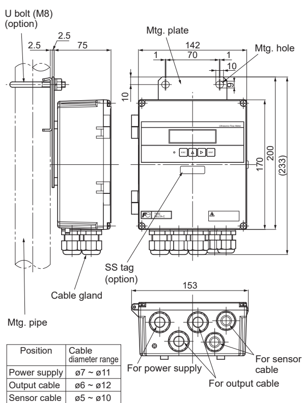
Flow transmitter : FSV...S (IP66)
