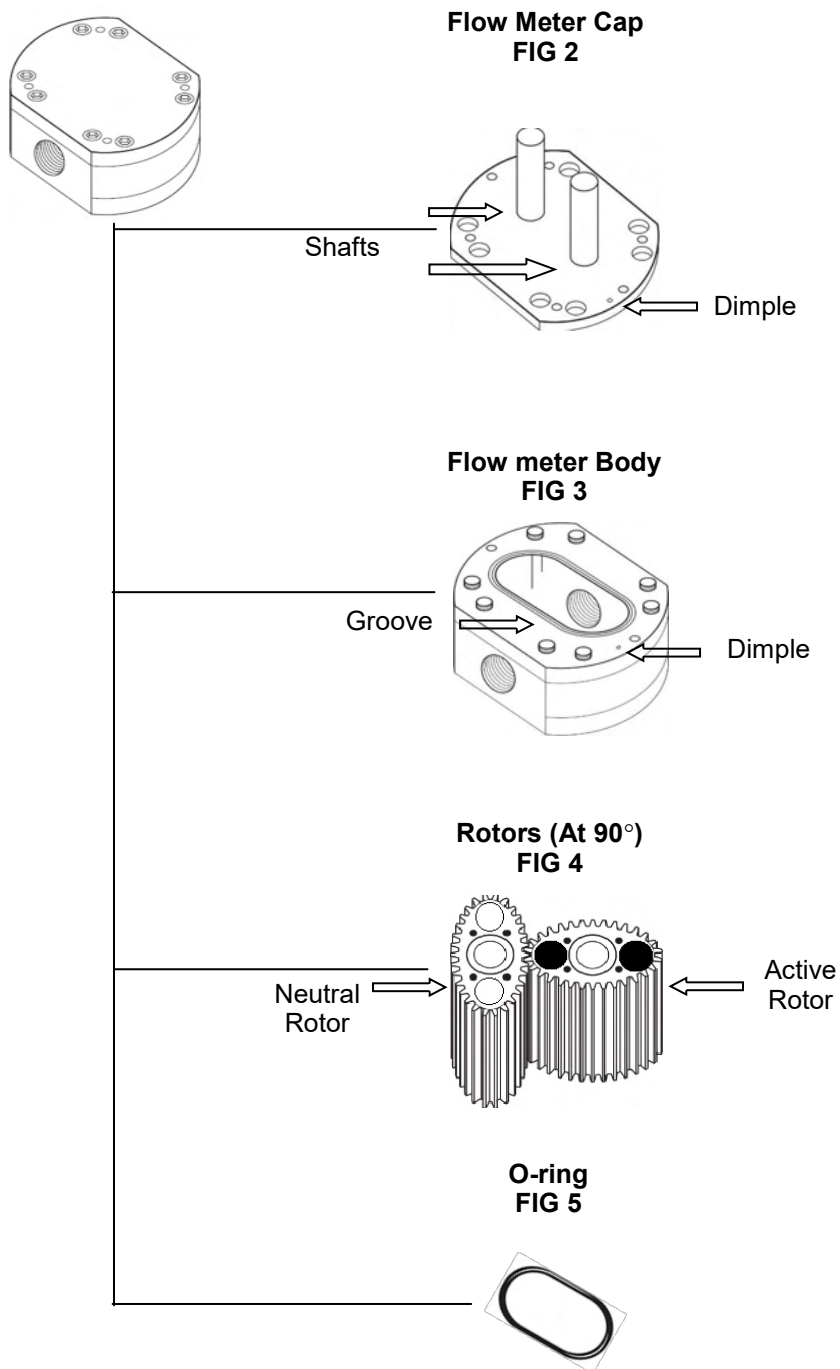
Flow meter FIG 1
