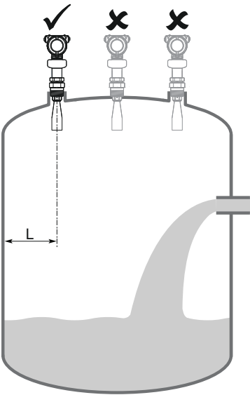
Figure 16: Recommended Mounting Position
